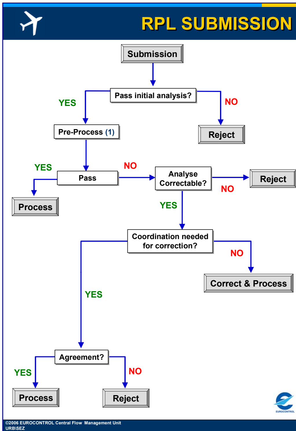
Figure 5-1 RPL Submission
