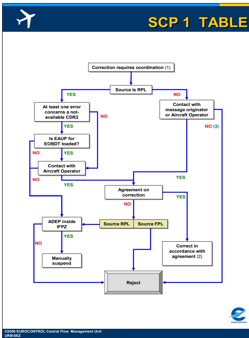
Figure 27-1 SCP1 Table
