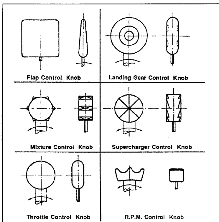
Figure 4-8. FAA requirements for cockpit control knobs (adapted from 14CFR, Ch. 1, Section 25.781)
