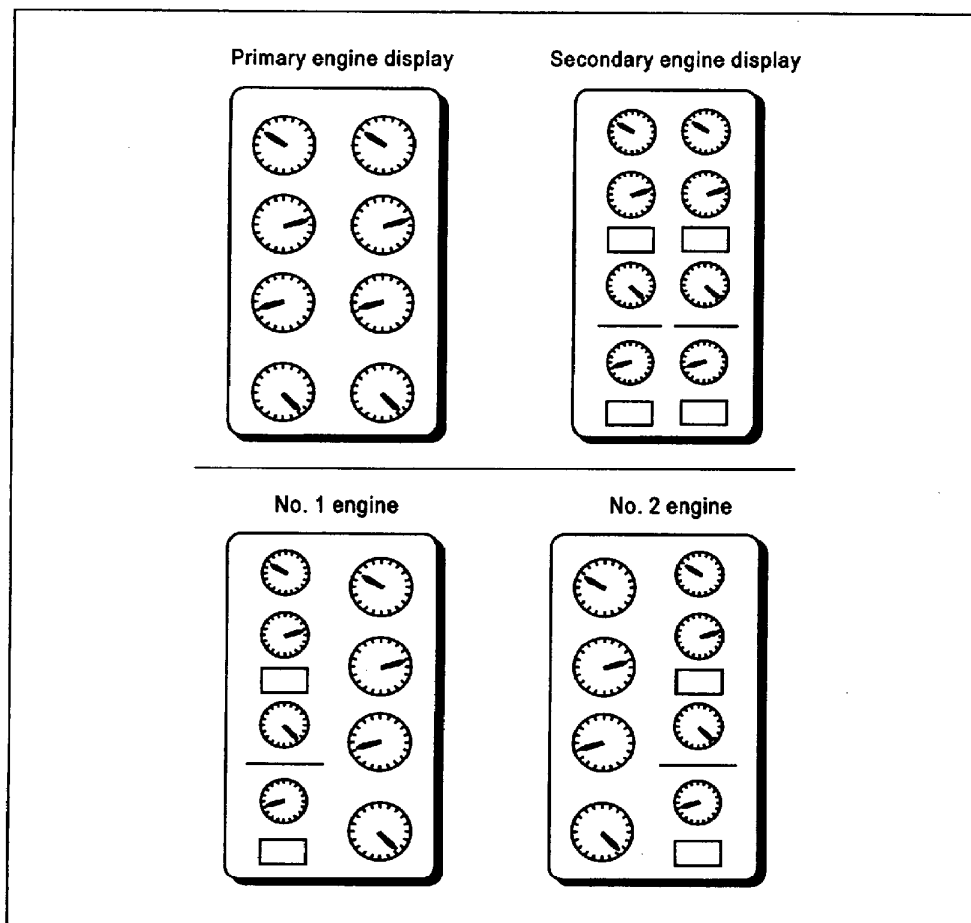
Figure 4-14. Proposed engine instrument system
