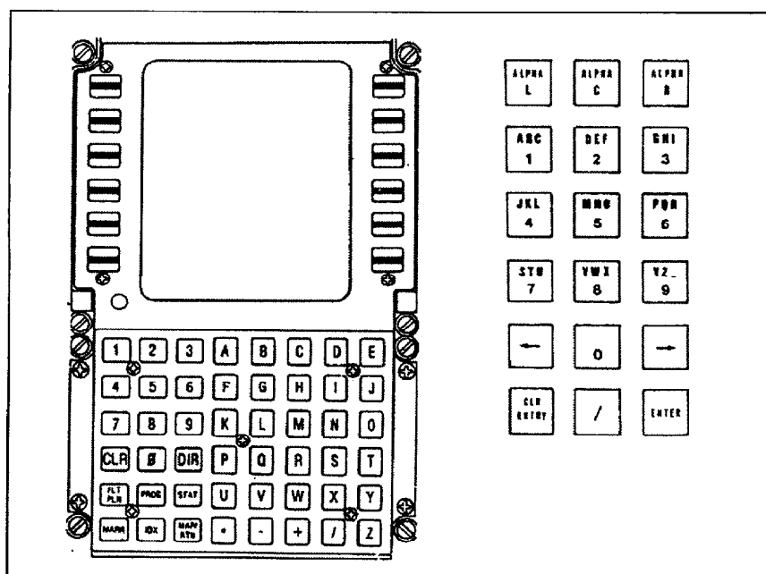
Figure 4-10. An example of a keyboard for a management or navigation system (left) and a suggested layout (adapted from Human Factors , L.C. Butterbaugh and T.H. Rockwell, 1982)
