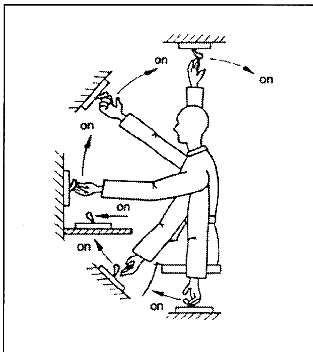
Figure 4-16. The “sweep-on” switch position concept which is slowly replacing the earlier “forward-on” arrangement (adapted from Human Factors in Flight , F.H. Hawkins, 1987)
