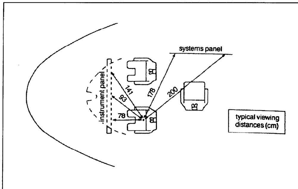
Figure 4-12. Typical viewing distances from the pilot's eye design eye position to various panels on the flight deck of a large jet (adapted from Human Factors in Flight , F.H. Hawkins, 1987)
