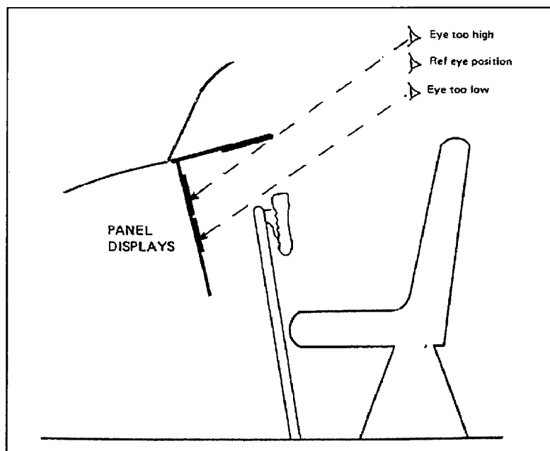
Figure 4-11. Reference eye position (adapted from Human Factors in Flight , F.H. Hawkins, 1987)
