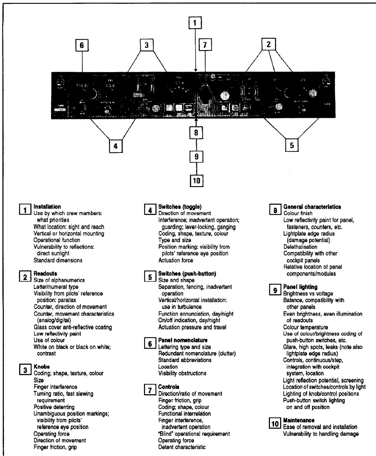
Figure 4-15. Checklist for evaluation of a typical cockpit panel
