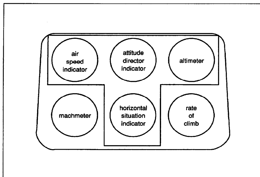
Figure 4-13. The "basic T panel" which forms the core of modern flight instrument panel layouts (adapted from Human Factors in Flight , F.H. Hawkins, 1987)
